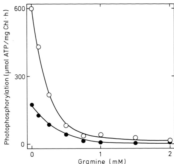
Fig. 1. Inhibition of cyclic and non-cyclic photophosphorylation in spinach thylakoid by gramine. Cyclic photophosphorylation (○) catalyzed by phenazine methosulfate and non-cyclic photophosphorylation (●) with methylviologen as electron acceptor were determined as described in the text. The reaction medium (1 ml) was 250 mM sucrose, 20 mM Tris-HCl (pH 7.8), 5 mM MgCl_2 , 2 mM ADP, 3 mM potassium phosphate containing 1 \times 10^6 cpm of ^{32}P , and either 50 \mu M phenazine methosulfate or 100 \mu M methylviologen and 500 \mu M NaN_3 . An amount of thylakoids equivalent to 10 \mu g of chlorophyll was used per test tube.
