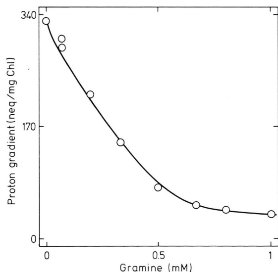
Fig. 3. Collapse of proton gradient by gramine. The pH changes of thylakoid suspensions were measured with a pH-meter equipped with a combination electrode and a recorder. The reaction medium (3 ml) was 10 mM NaCl, 50 \mu M phenazine methosulfate, and thylakoids 150 \mu g of chlorophyll, prepared as usual but washed and resuspended in 10 mM NaCl.
